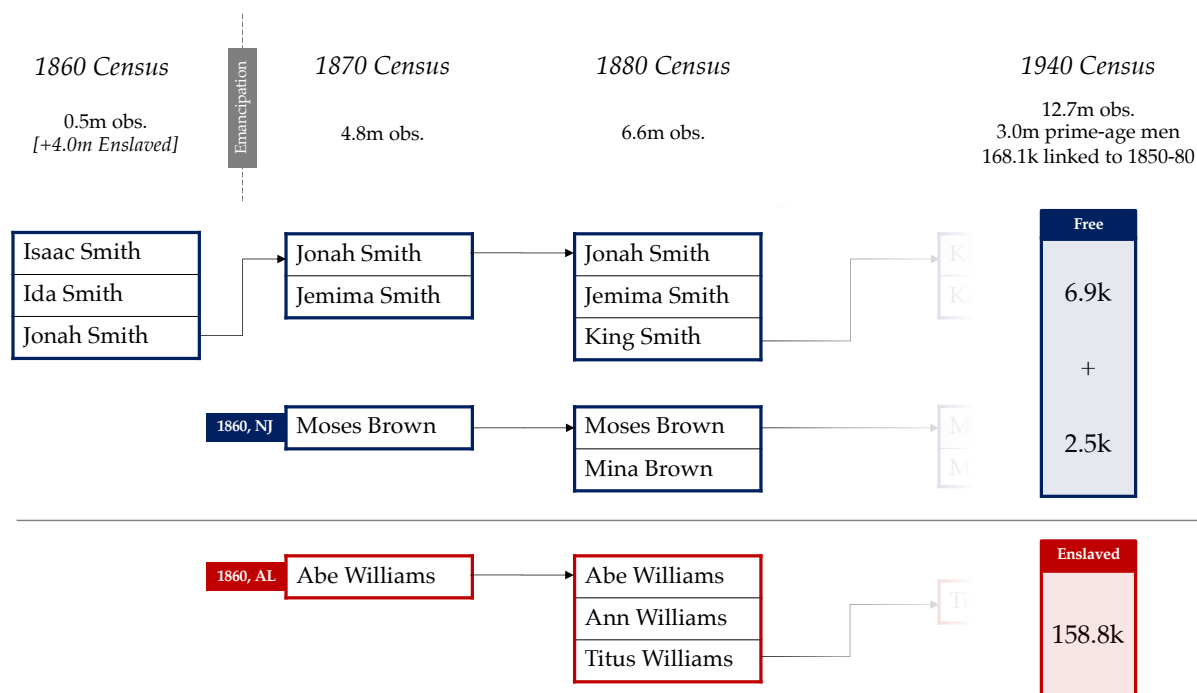
FIGURE C.42: Illustration of Our Free-Enslaved Classification Algorithm
