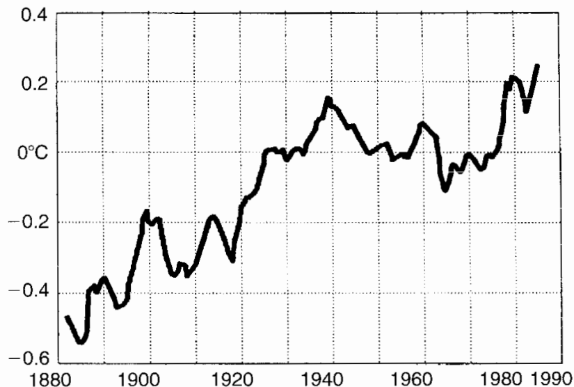
Figure 1. Changes in the global surface air temperature since 1880 (referred to the average temperature for 1951 to 1980). Note the rapid rise up to about 1940, likely the recovery from the “Little Ice Age” that followed the “Medieval Climate Optimum.” Temperatures fell till about 1975, when there was a sudden jump, tied to changes in ocean circulation and other worldwide changes. The climate record since 1979 has been in controversy, with surface observations indicating a warming while satellite and balloon-borne radiosondes showed no warming of the bulk of the atmosphere. This disparity has not yet been satisfactorily explained. See the National Research Council, Reconciling Observations of Global Temperature Change (Washington, D.C.: National Academy Press, 2000).
